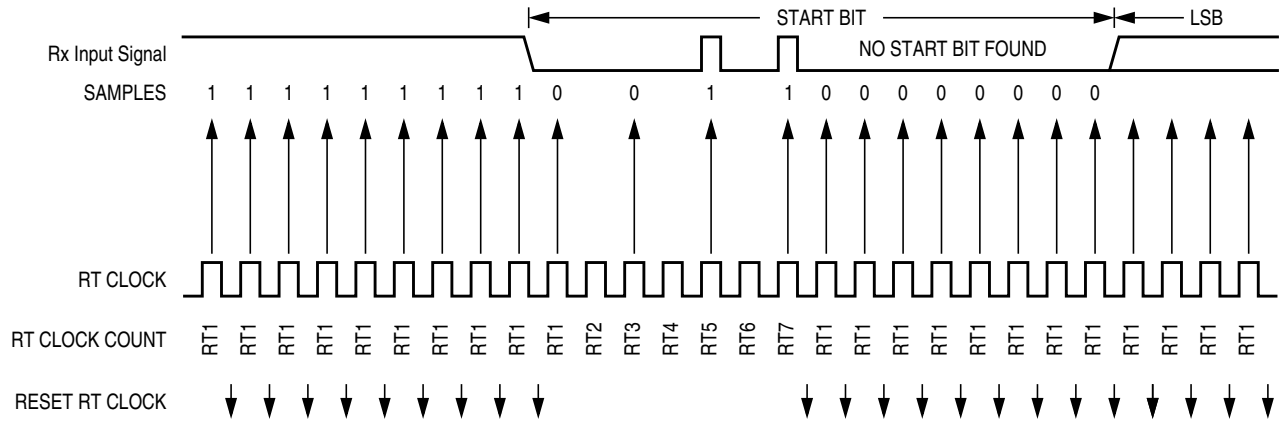
Figure 1-18. Start Bit Search Example 5
