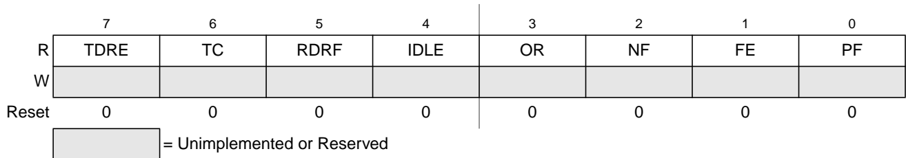
Figure 1-6. SCI Status Register 1 (SCISR1)
