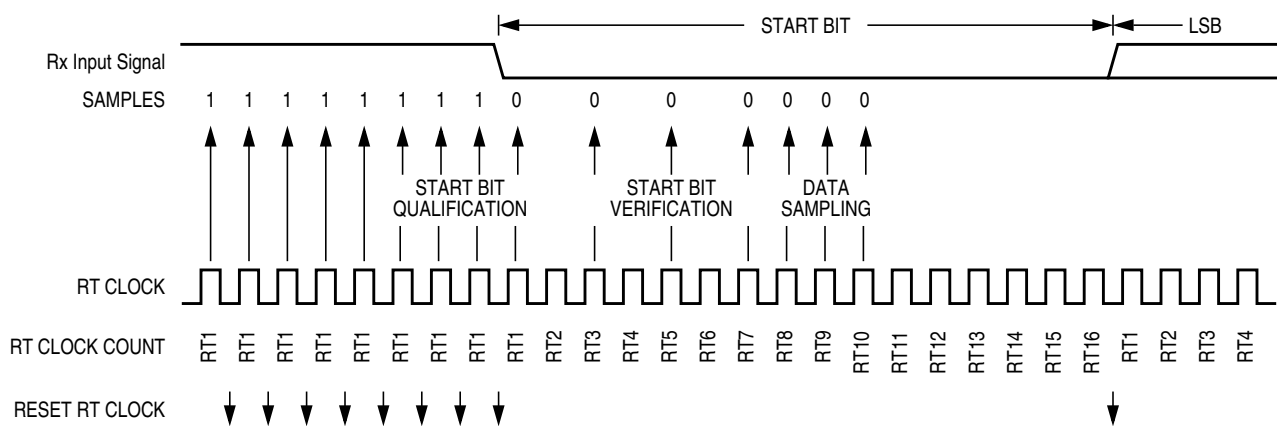
Figure 1-13. Receiver Data Sampling
