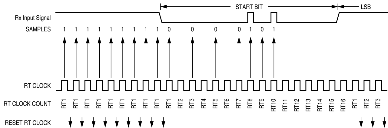
Figure 1-19. Start Bit Search Example 6
