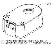
H-OPTION COVER (COVER HOLE FOR EXTENDED SHAFT LENGTHS)
