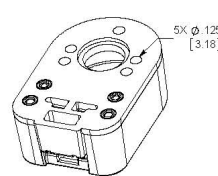
3-OPTION BASE (LARGER MOUNTING HOLES)
