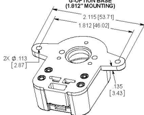
G-OPTION BASE (1.812" MOUNTING)
