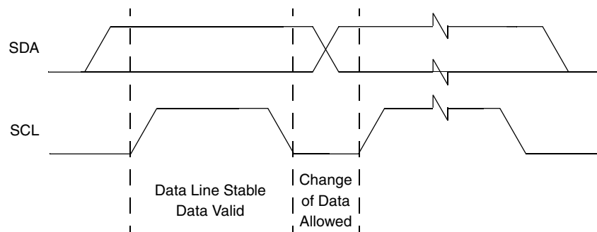
Figure 1. Bit Transfer
