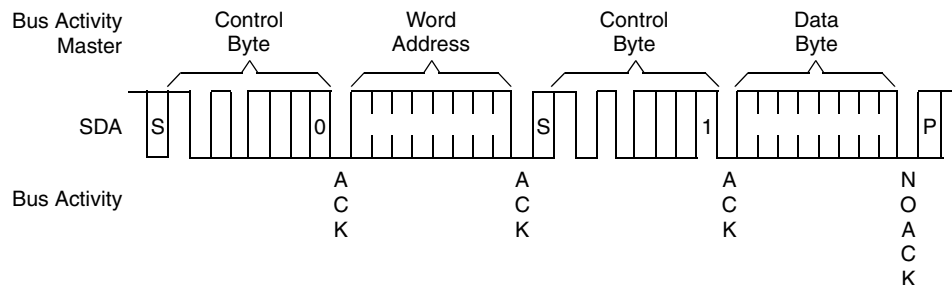
Figure 6. Read-Operation Structure
