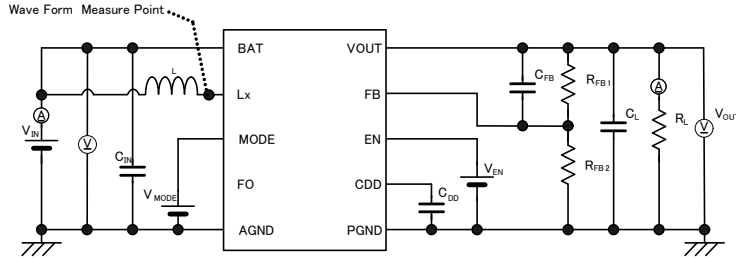
< Circuit No.2 >
