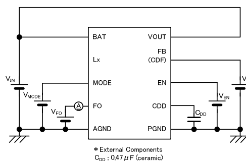
< Circuit No.7 >
