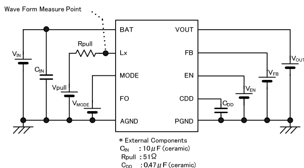
< Circuit No.6 >
