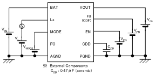
< Circuit No.4 >
