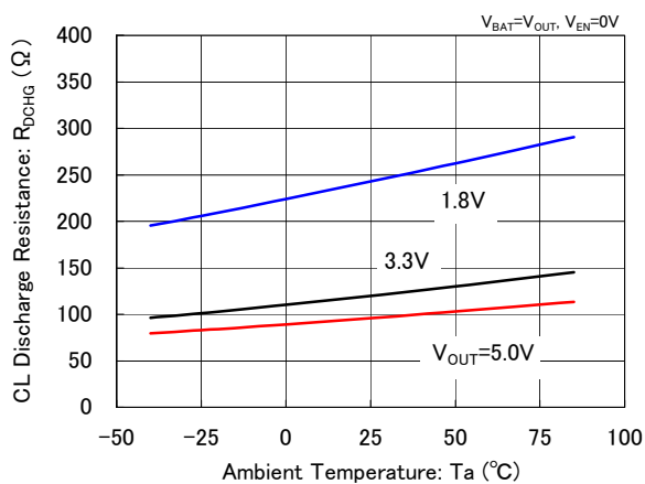
XC9131F05C
