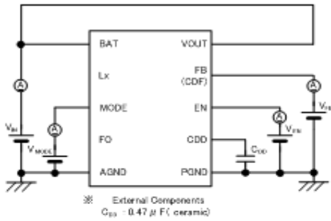
< Circuit No.2 >
