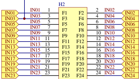
INPUT FIELD HEADER, 24 PIN (Connects to signals, sensors, or actuator lines)
