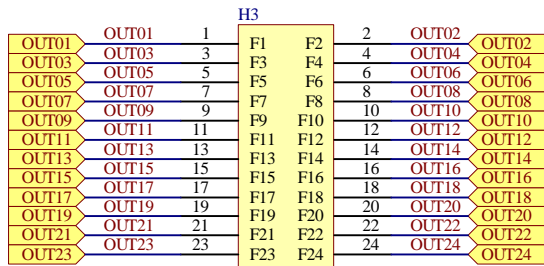
OUTPUT FIELD HEADER, 24 PIN (Connects to the Field Header of the other Wildcard)
