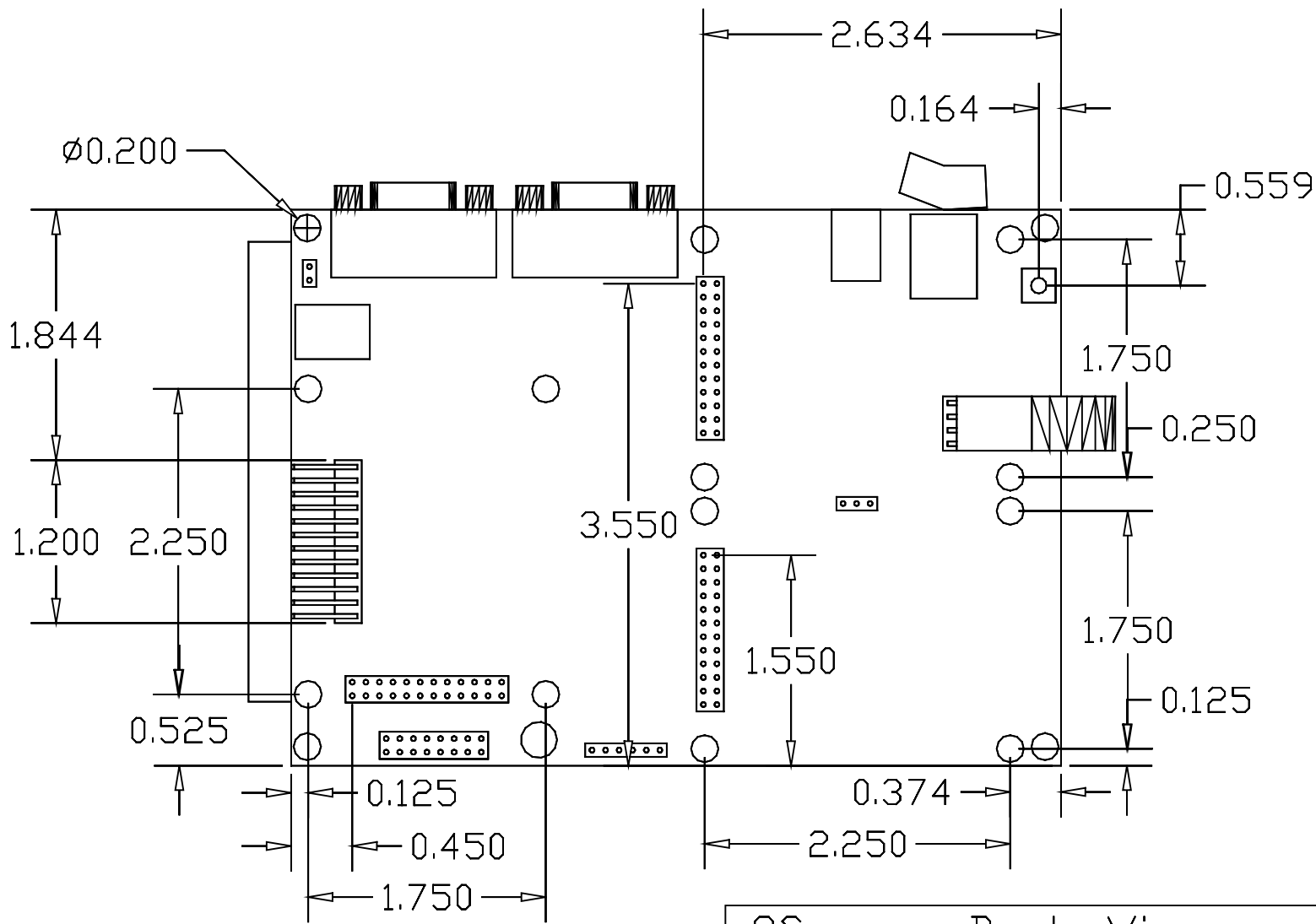
QScreen Back View Mosaic Industries, Inc. www.mosaic-industries.com
